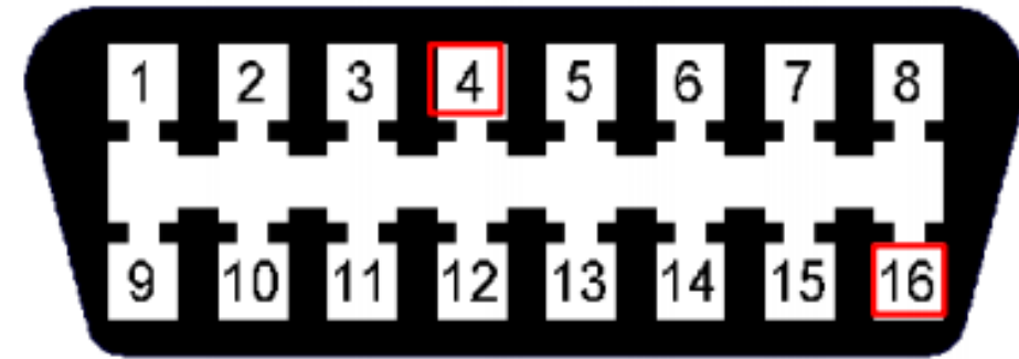
Figure 1 (OBD 2 Connector)
