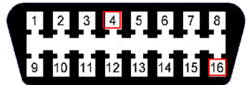
Figure 1 (OBD 2 Connector)
