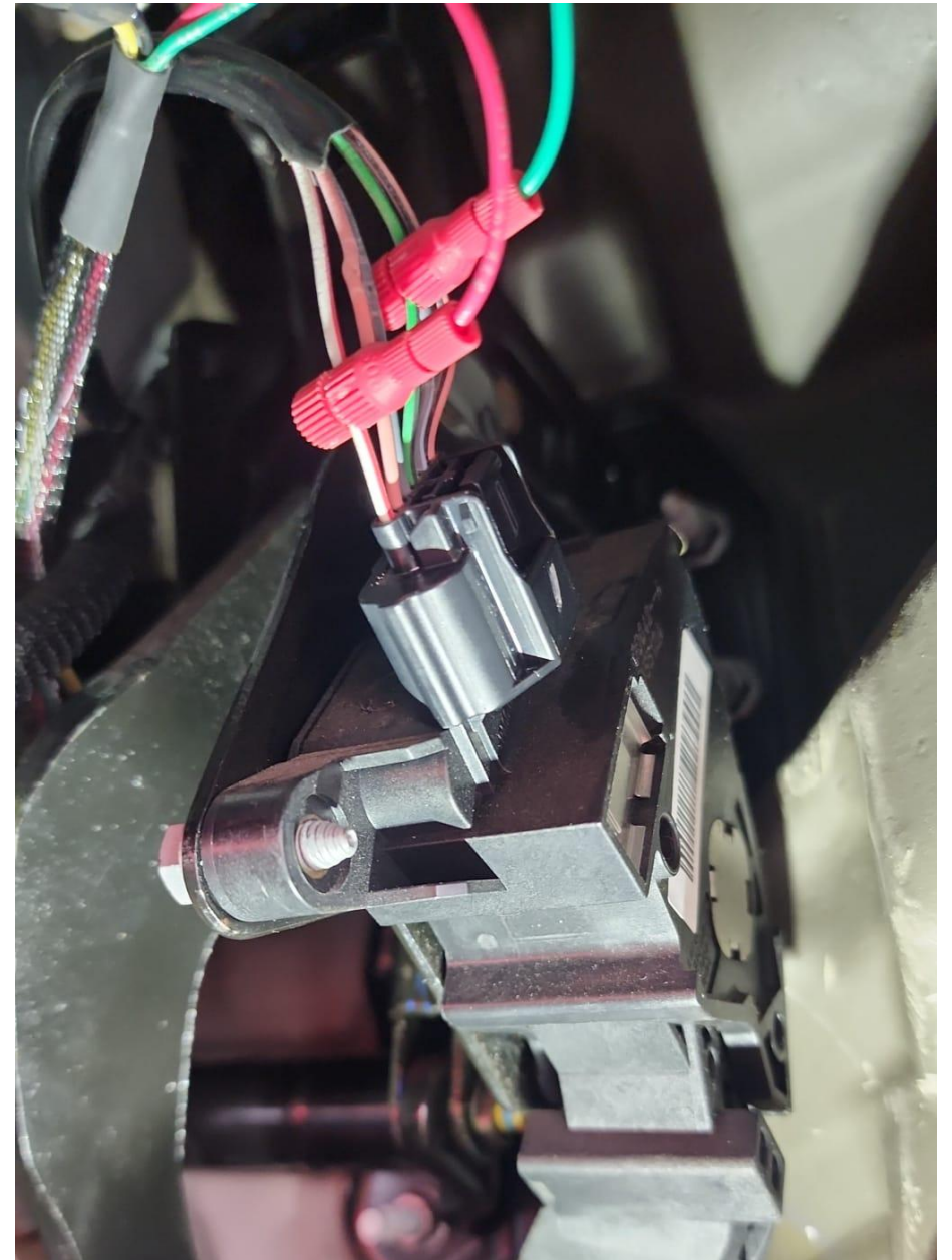
Accelerator Pedal Position Sensor (APPS)
