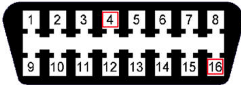
Figure 5 - OBD2 port connections for power and ground connections)
