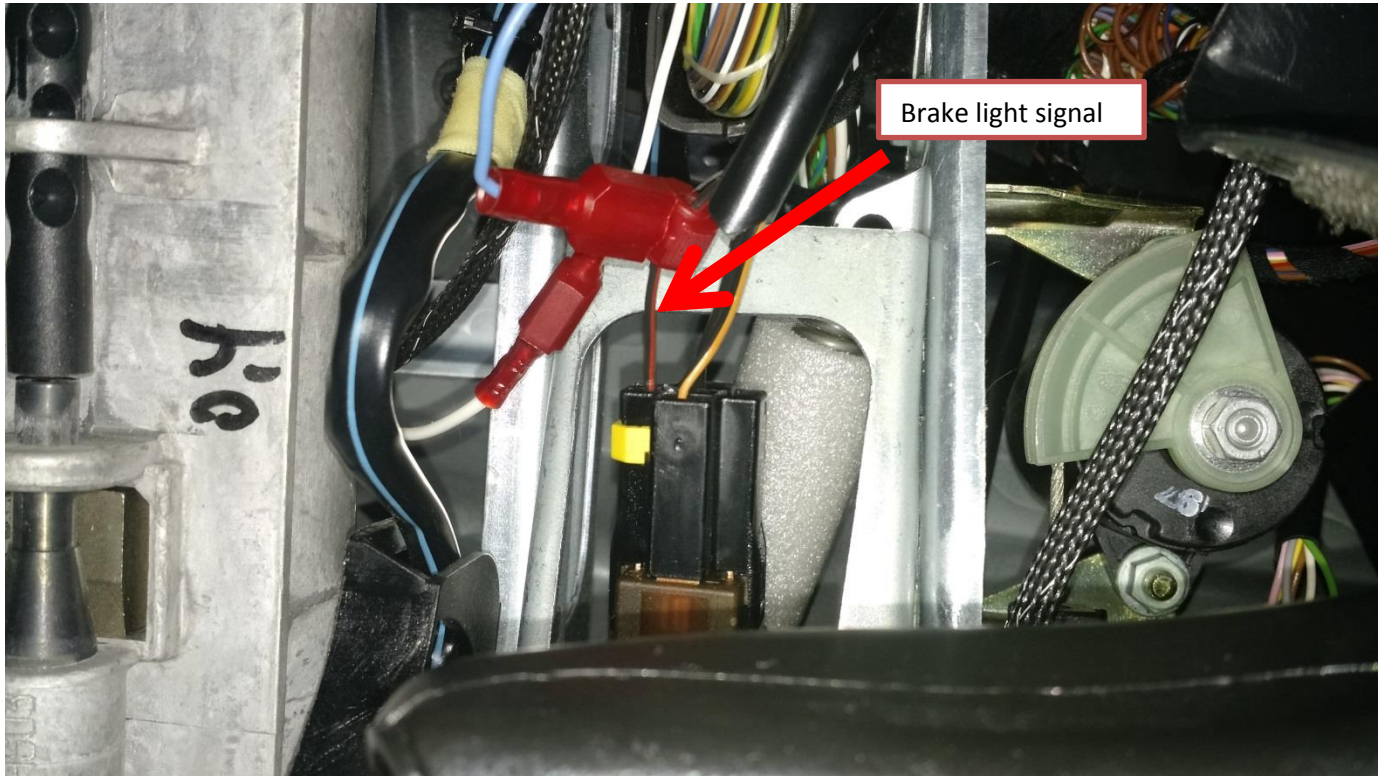
Figure 3 (Brake pedal switch connection)
