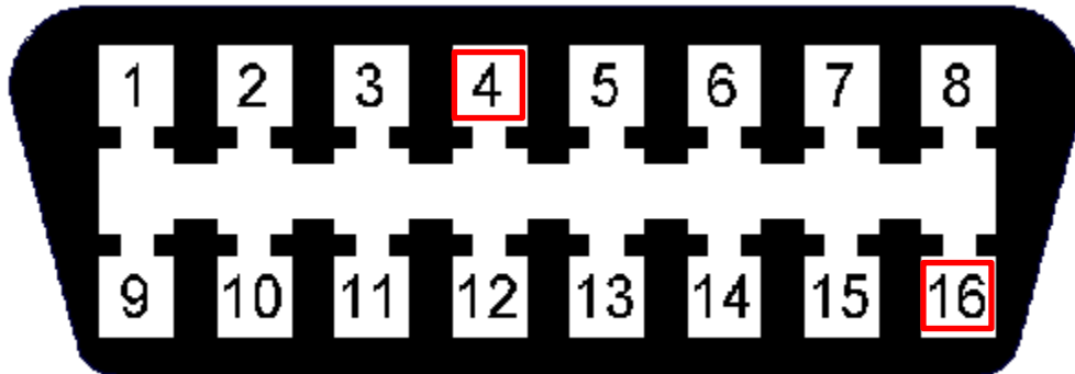
Figure 3 (OBD 2 Connector)
