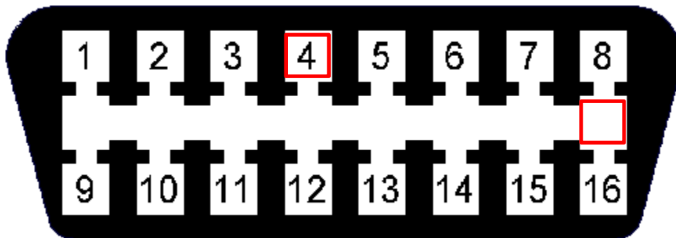
Figure 2 (OBD 2 Connector)
