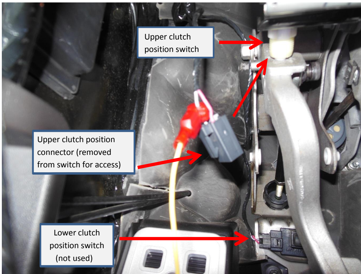
Figure 5 (Clutch position switch)
