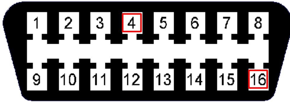
Figure 4 (OBD2 Ground and 12V connections)
