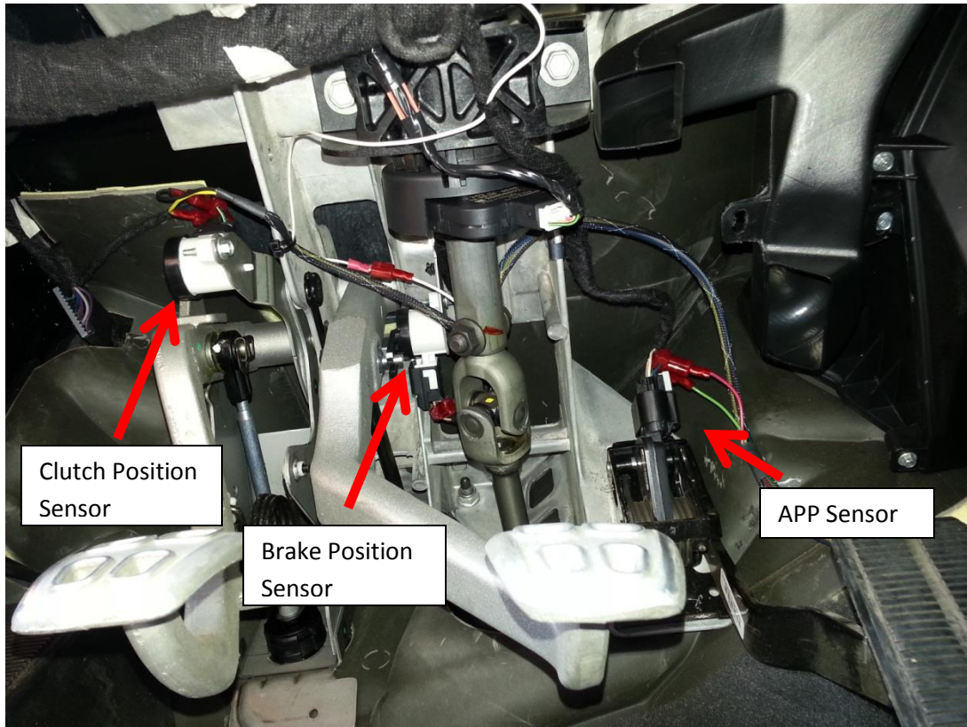
Figure 2 (Sensor Locations)
