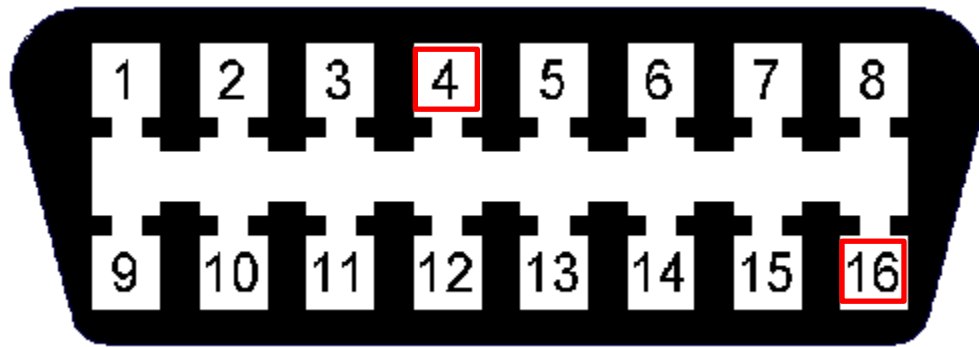
Figure 2 (OBD 2 Connector)
