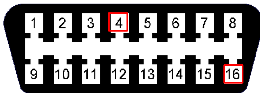
Figure 1 (OBD 2 Connector)
