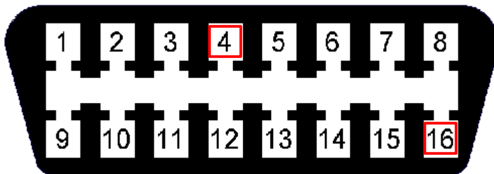
Figure 1 (OBD 2 Connector)
