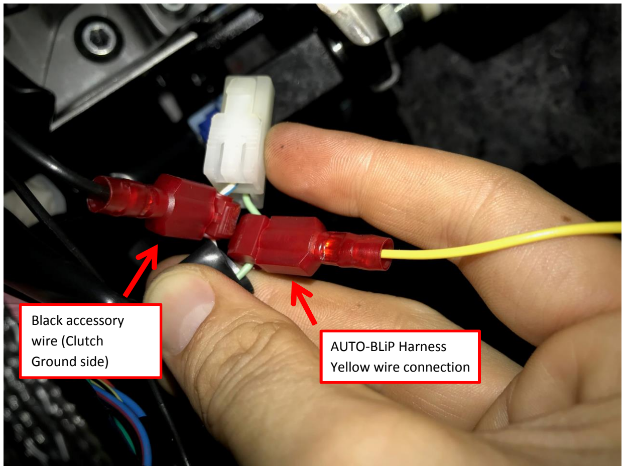
Figure 8 (Clutch pedal sensor wire connections)
