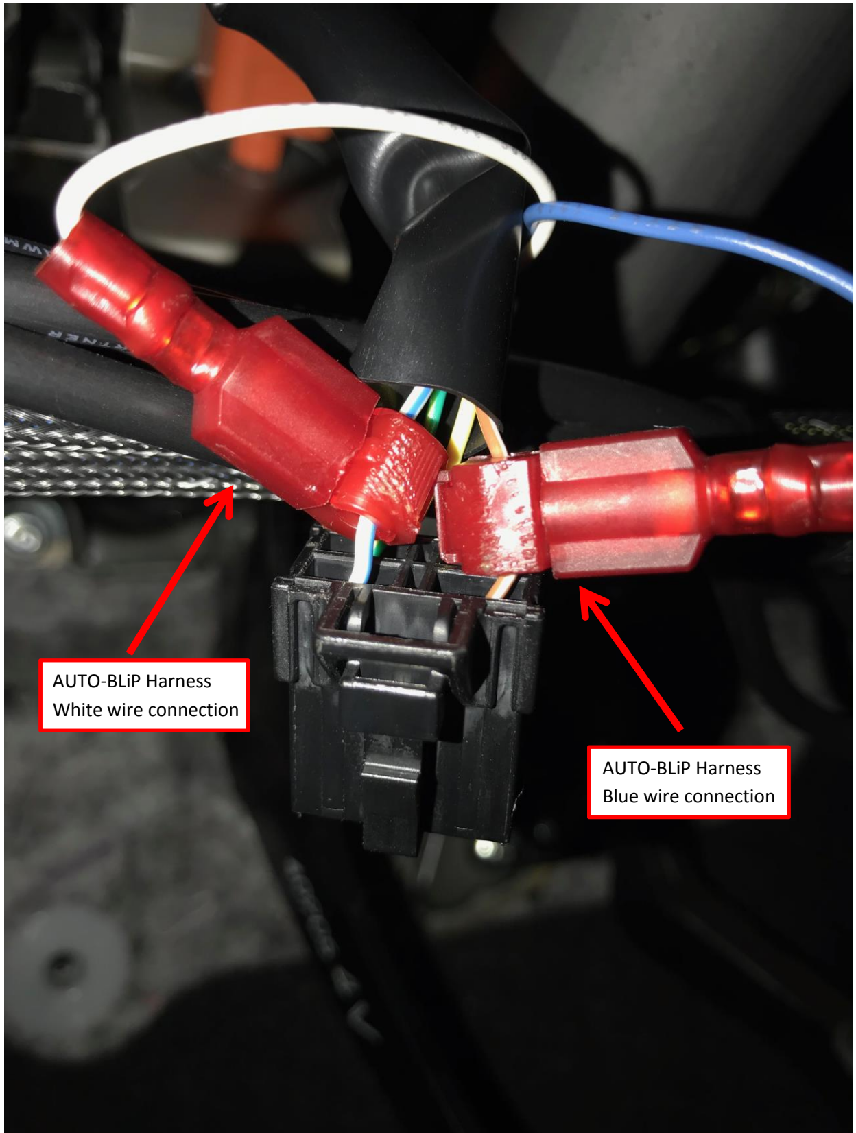
Figure 7 (Brake pedal sensor connections)
