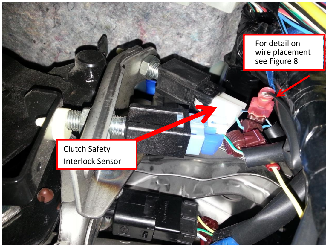
Figure 2 (Clutch Sensors - general location; for detail see Figure 8)
