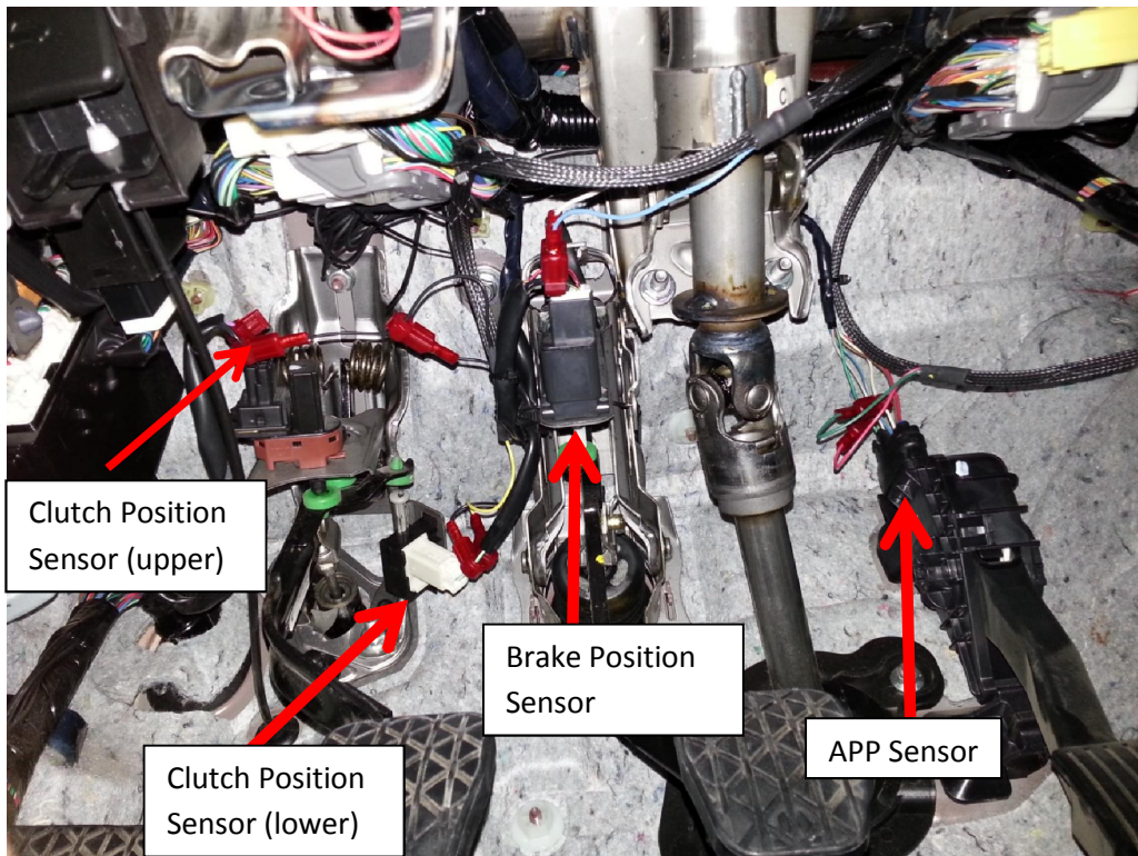
This picture is for GENERAL sensor locations only (not specific to MX-5 ND)
