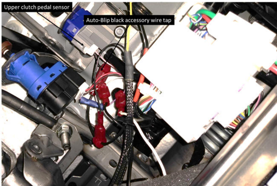
Figure 5 (Upper Clutch Sensor wiretap placement) Picture shows different connectors than Posi-taps *Auto-Blip Black accessory wire connection: Use voltmeter to test for GROUND at tapped car wire
