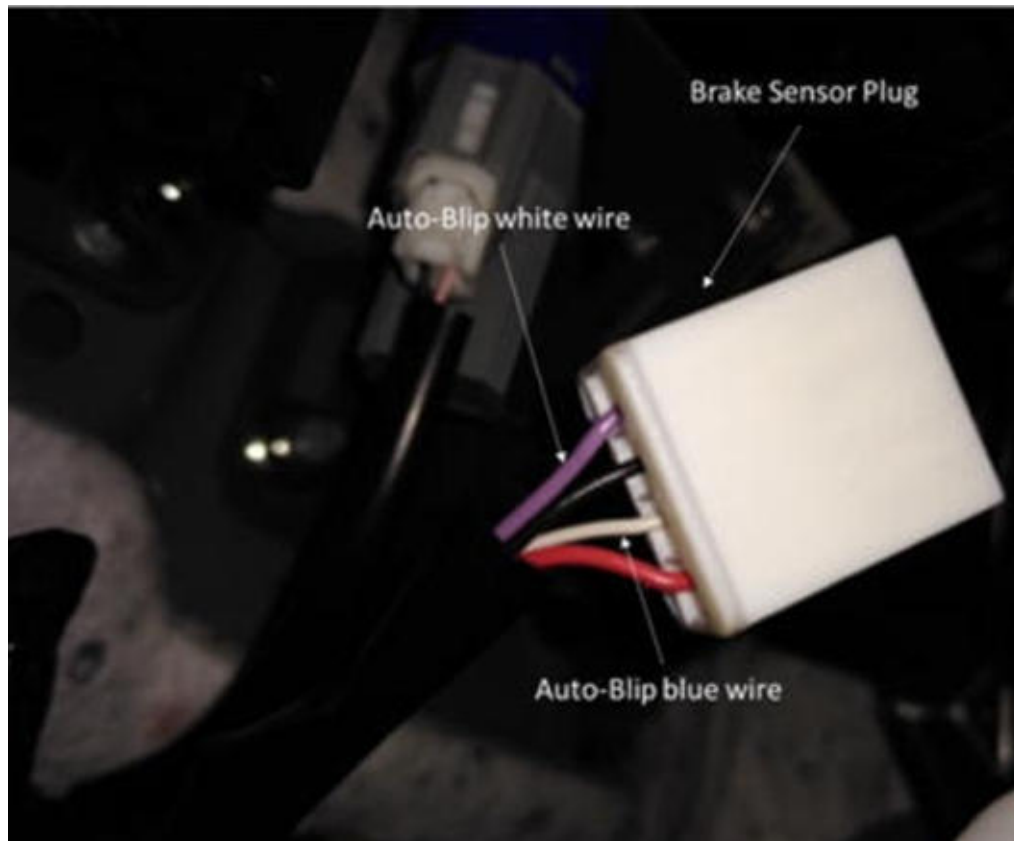
Figure 3 (Brake Sensor wire taps placement*) This picture not specific to Miata ND
