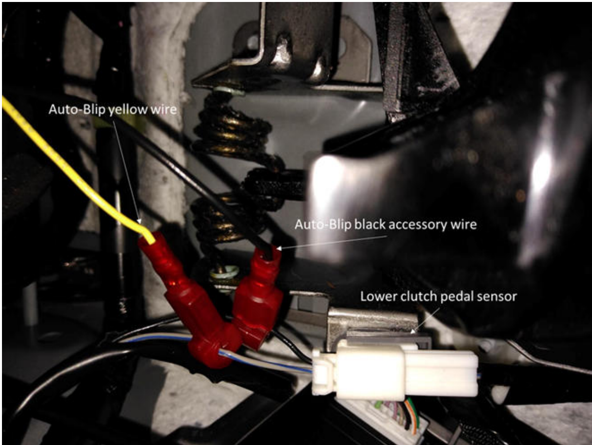
Figure 4 (Lower Clutch Sensor wire taps placement) This picture not specific to Miata ND *Auto-Blip Black accessory wire connection: Use voltmeter to test for GROUND at tapped car wire
