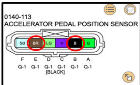
Figures 2, 2B, 2C (Accelerator Pedal Position Sensor wire taps placement) These pictures are specific to ND
