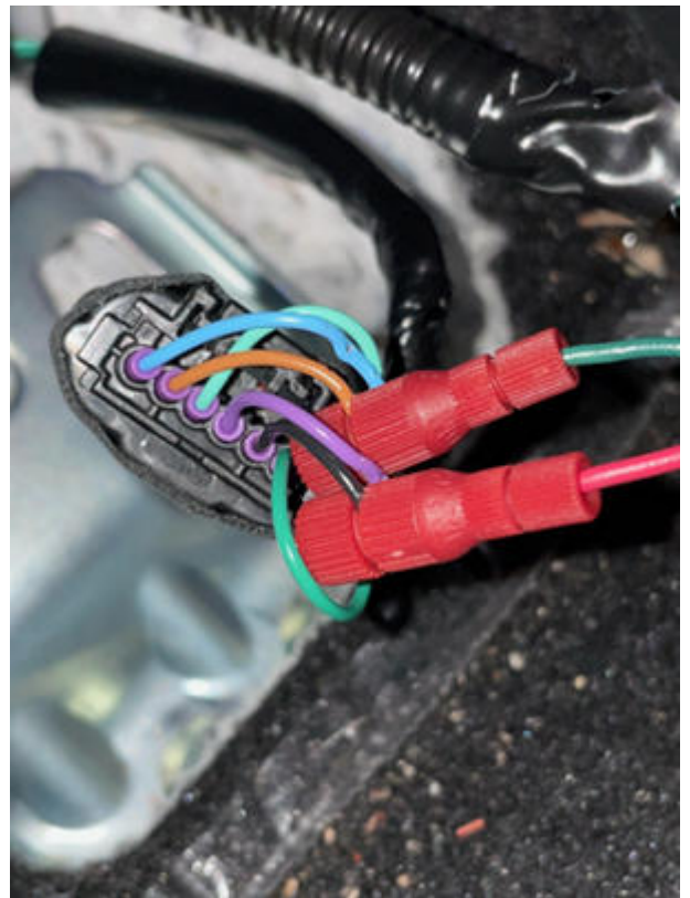
Figures 2, 2B, 2C (Accelerator Pedal Position Sensor wire taps placement) These pictures are specific to ND
