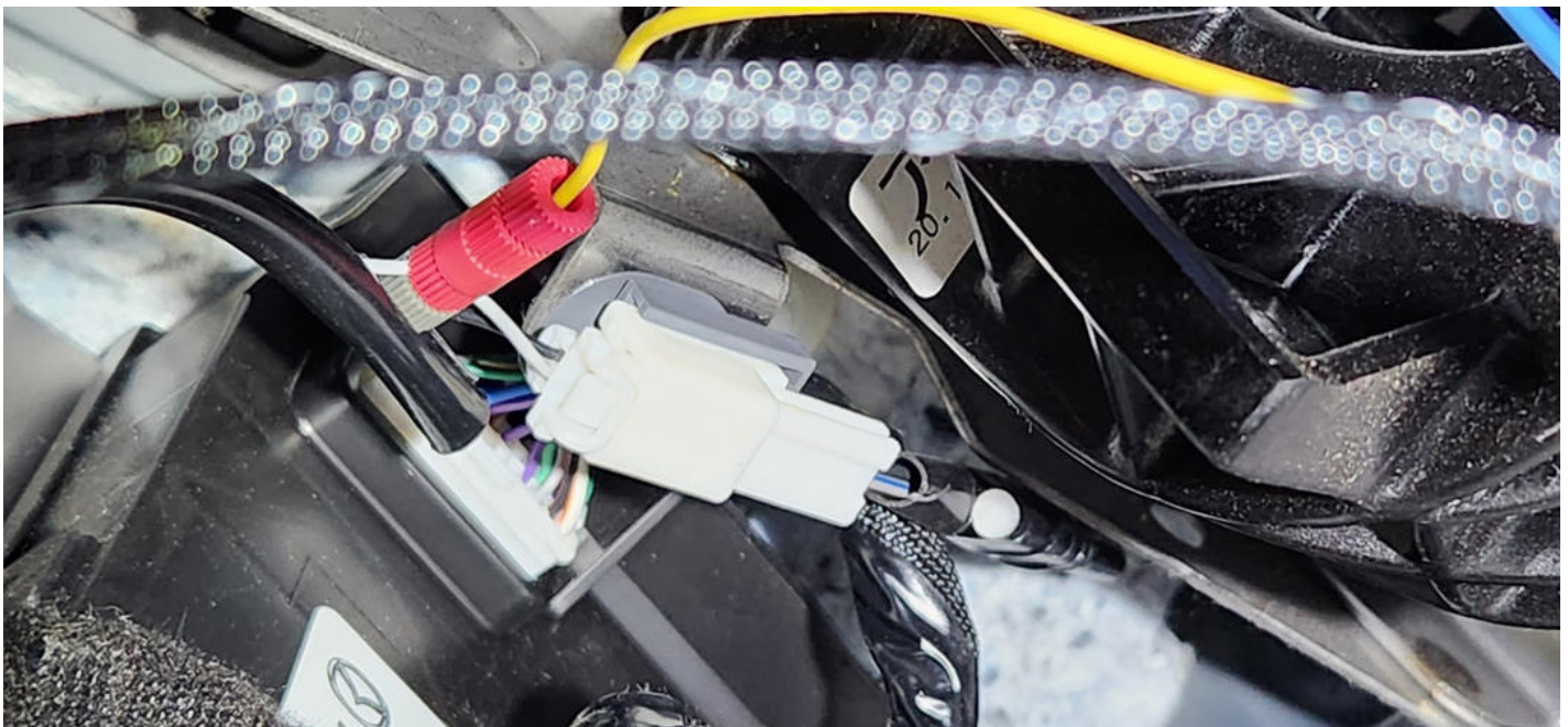
Figure 4B - Lower Clutch Sensor wire tap placement* (safety interlock switch ) This picture is specific to Miata ND *Use voltmeter to test; voltage present only when clutch is pressed (safety interlock switch brake light wire)
