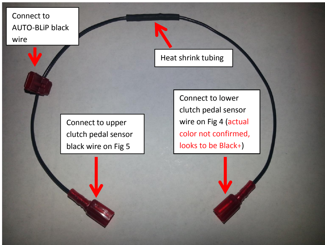
Figure 6 (Black accessory wire)
