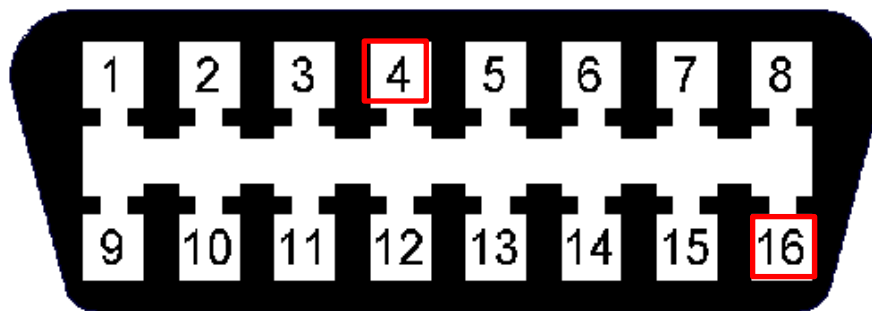
Figure 1 (OBD 2 Connector)
