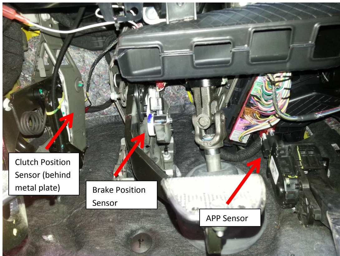
Figure 1 (Sensor Locations)
