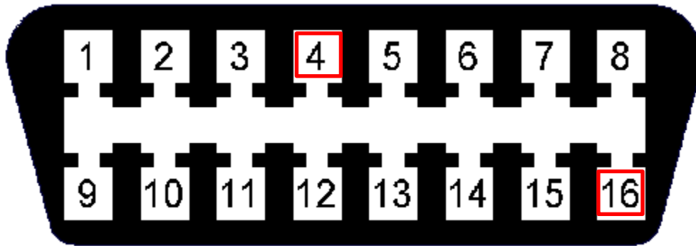
Figure 8 (OBD 2 Connector)
