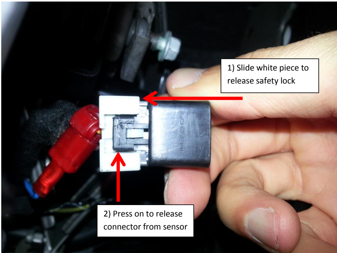
Figure 3 (Clutch & Brake connector)
