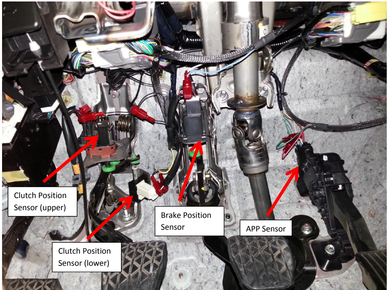
Figure 1 - General sensor locations (picture for illustration purposes only, not specific to MX-5 ND)
