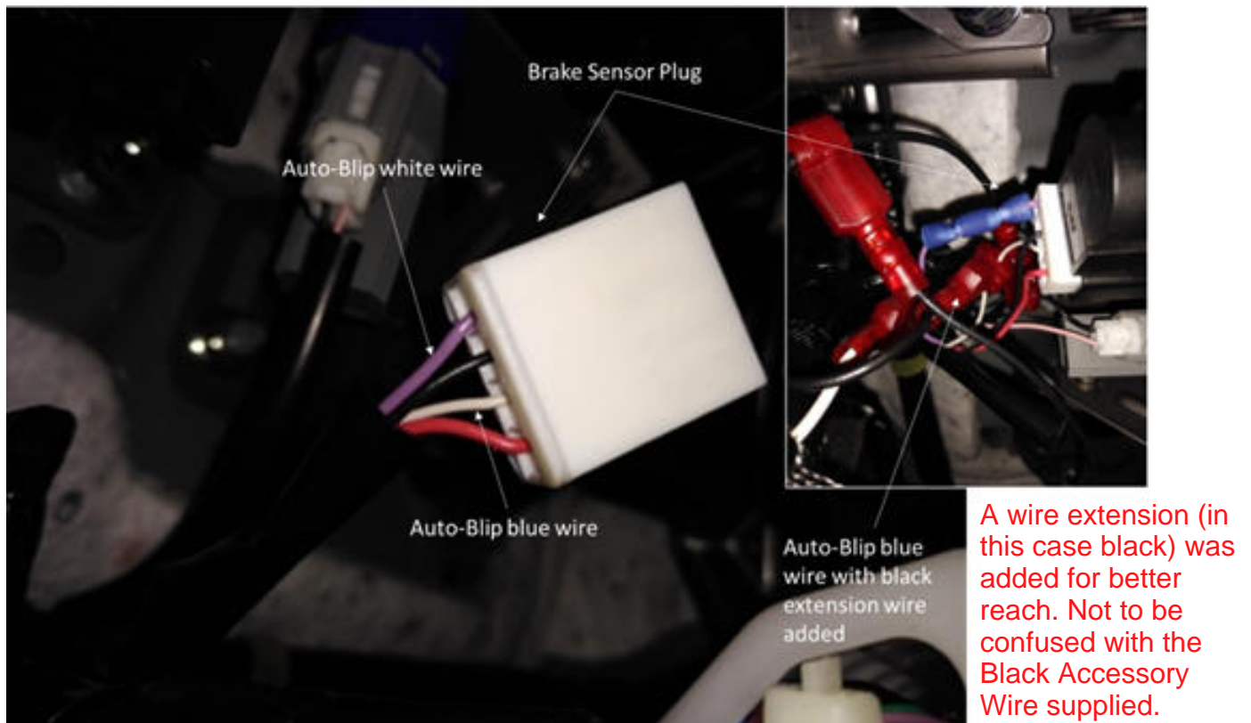
Figure 3 (Brake Sensor wire taps placement)
