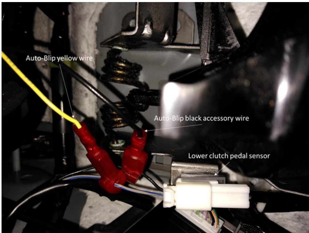
Figure 4 (Lower Clutch Sensor wire taps placement)
