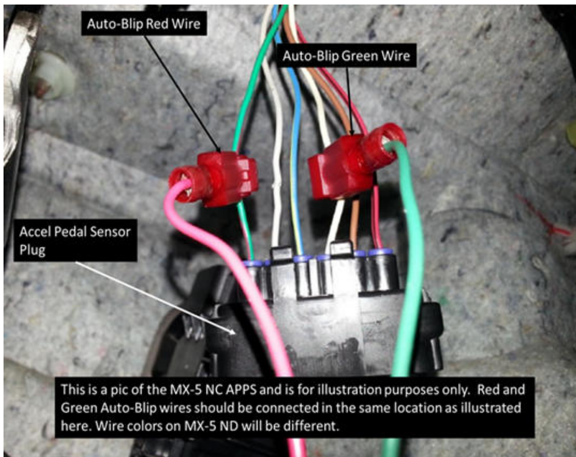
Figure 2 (Accelerator Pedal Position Sensor wire taps placement)
