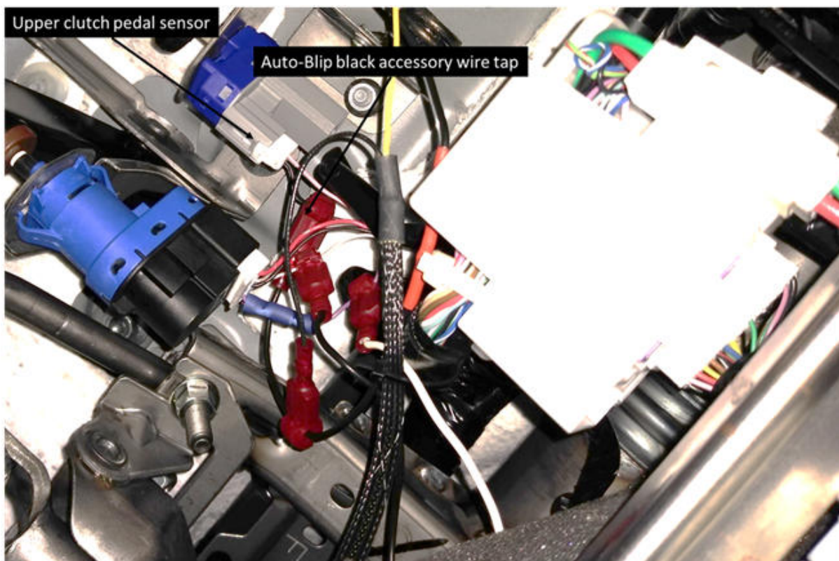
Figure 5 (Upper Clutch Sensor wiretap placement)
