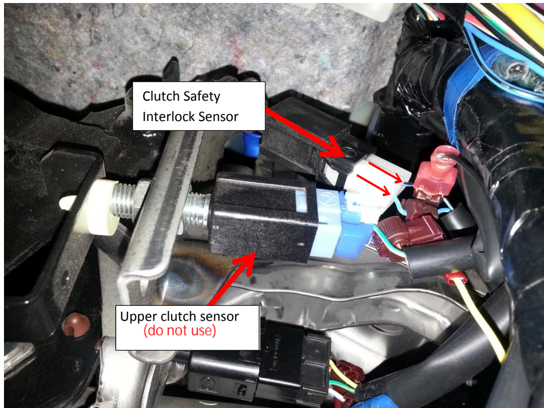
Figure 2 (Clutch Sensors)
