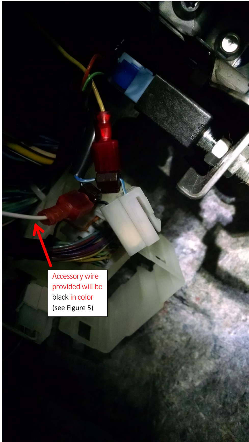
Figure 8 (Clutch pedal sensor wire connections)
