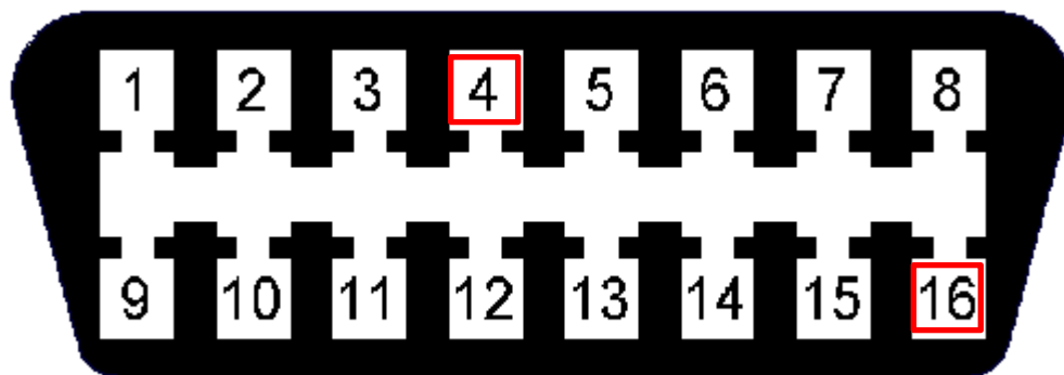
Figure 1 (OBD 2 Connector)
