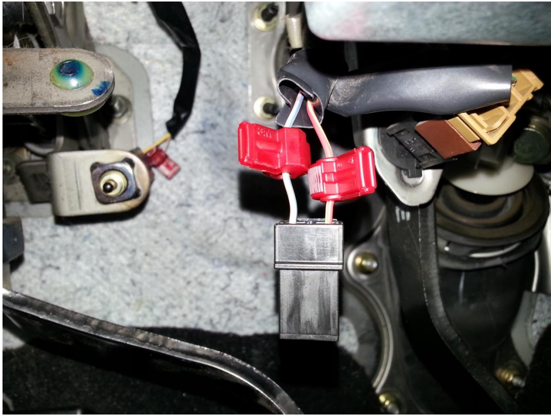
Figure 4 (Brake Sensor wire tabs placement)
