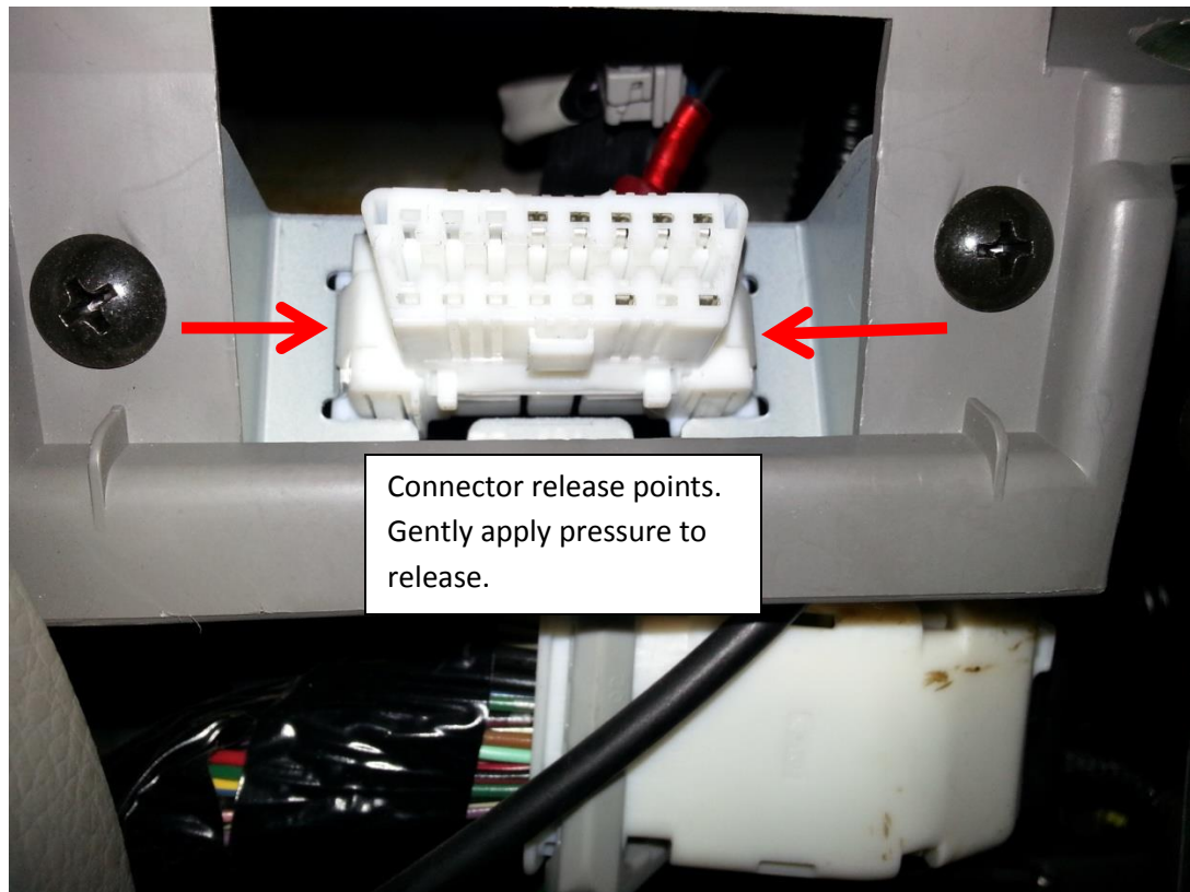
Figure 6 (OBDII Connector)
