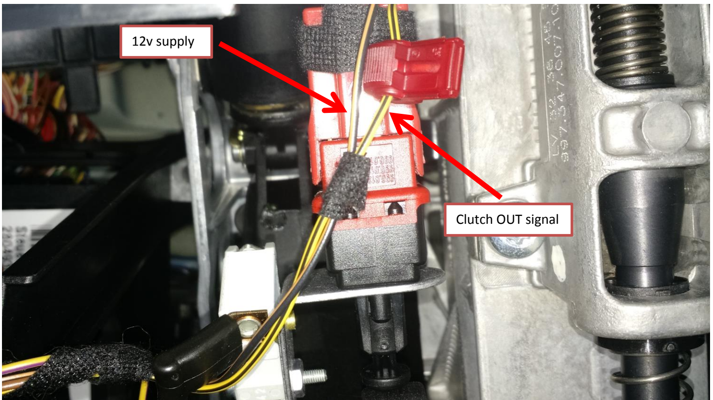
Figure 4b (Clutch pedal OUT Switch connection)
