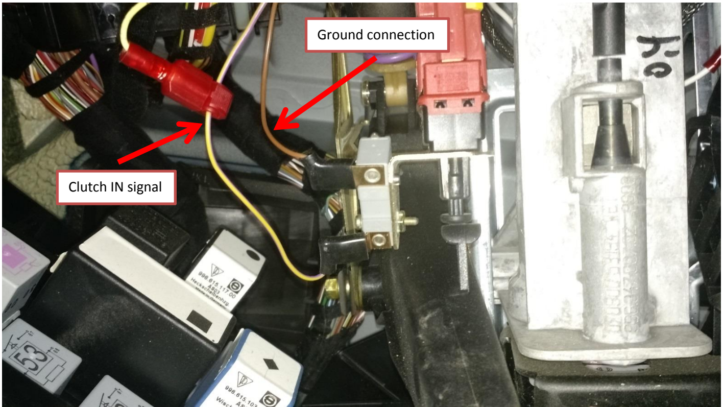
Figure 4a (Clutch pedal IN Switch connection)
