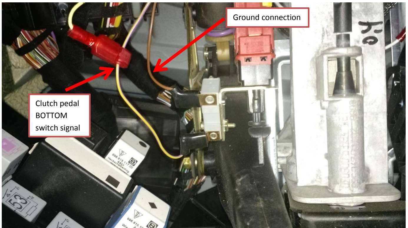
Figure 4 (Clutch pedal BOTTOM Switch connection)
