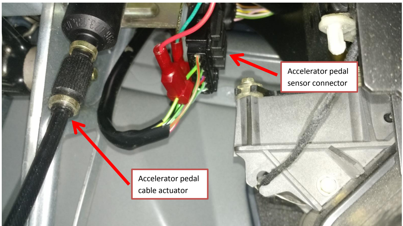
Figure 2a (Accelerator Pedal Position Sensor connections)
