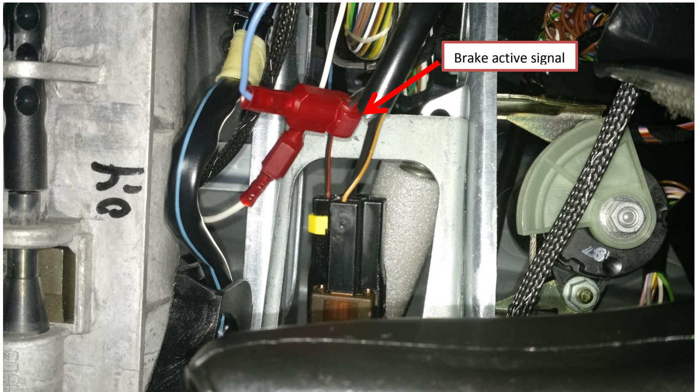
Figure 3 (Brake pedal switch connection)
