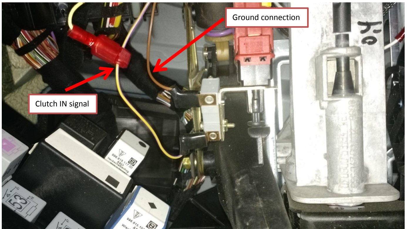
Figure 4 (Clutch pedal IN Switch connection)
