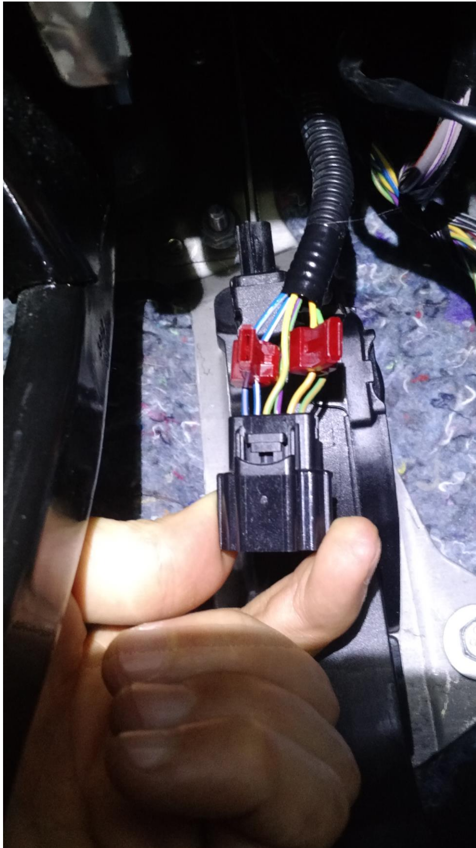
Figure 3 (Accelerator pedal position sensor connector)
