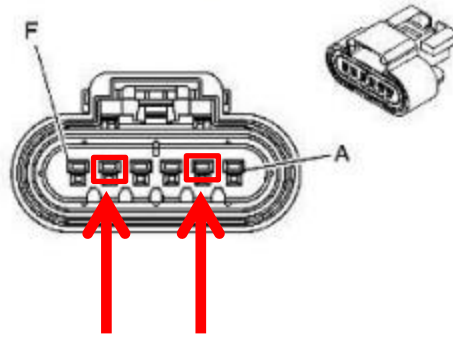
Figure 4 (Accelerator pedal connection placement)
