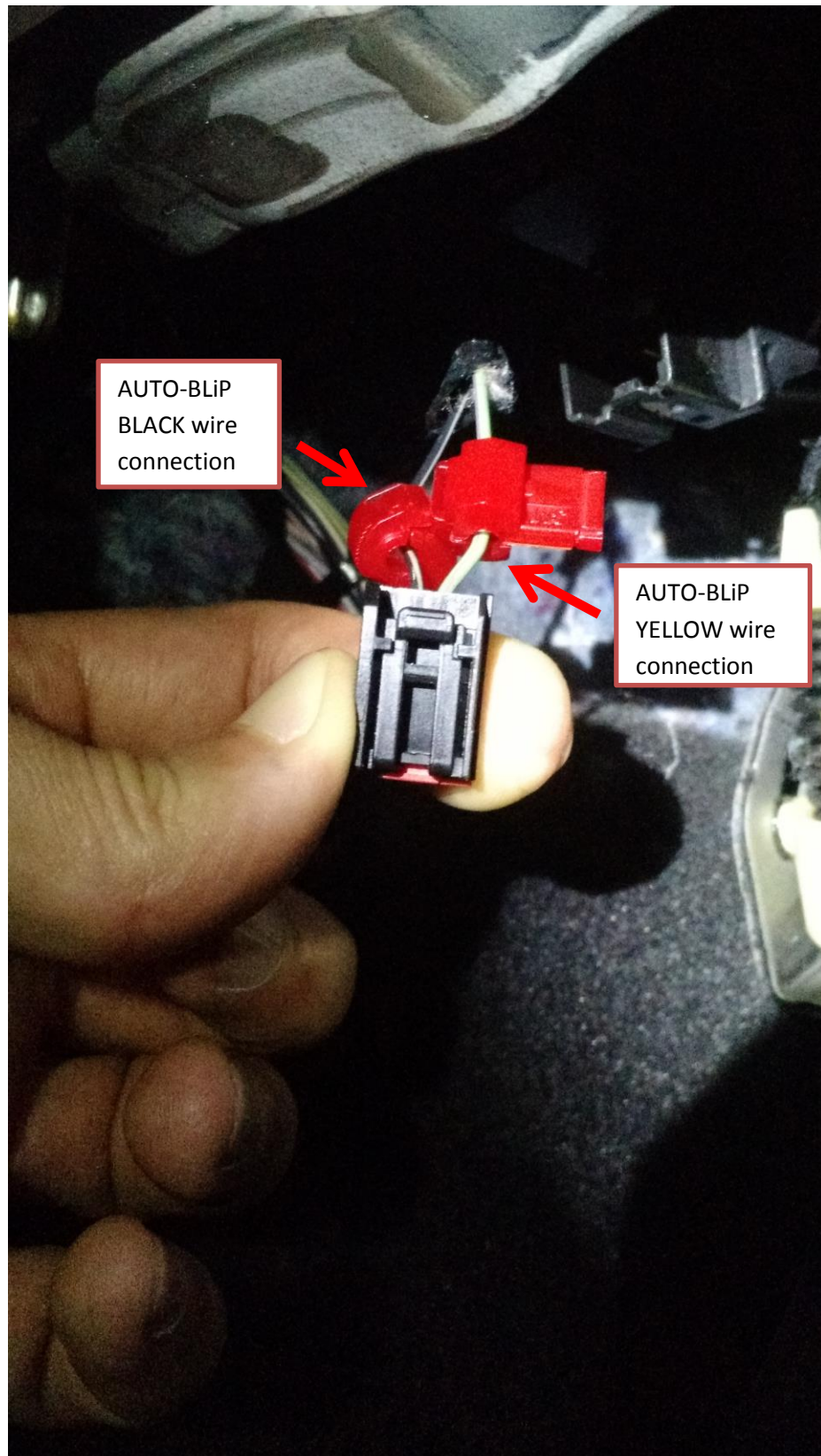
Figure 1 (Clutch pedal cruise control disable switch connector)
