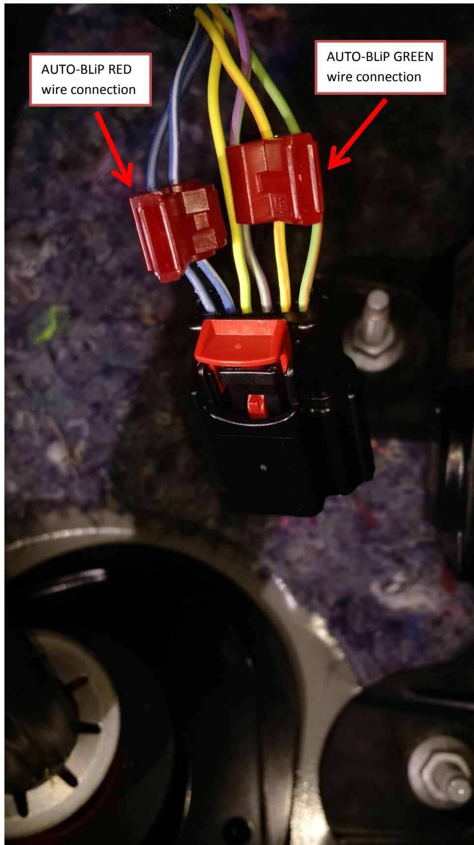
Figure 3 (Accelerator pedal sensor connector)
