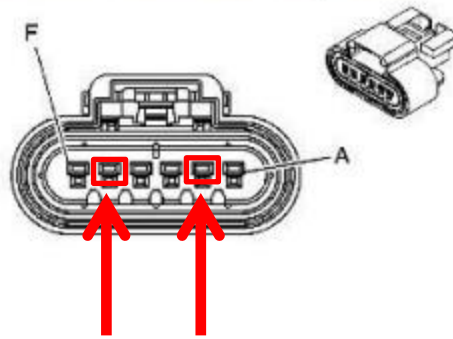
Figure 4 (Accelerator pedal connection points)
