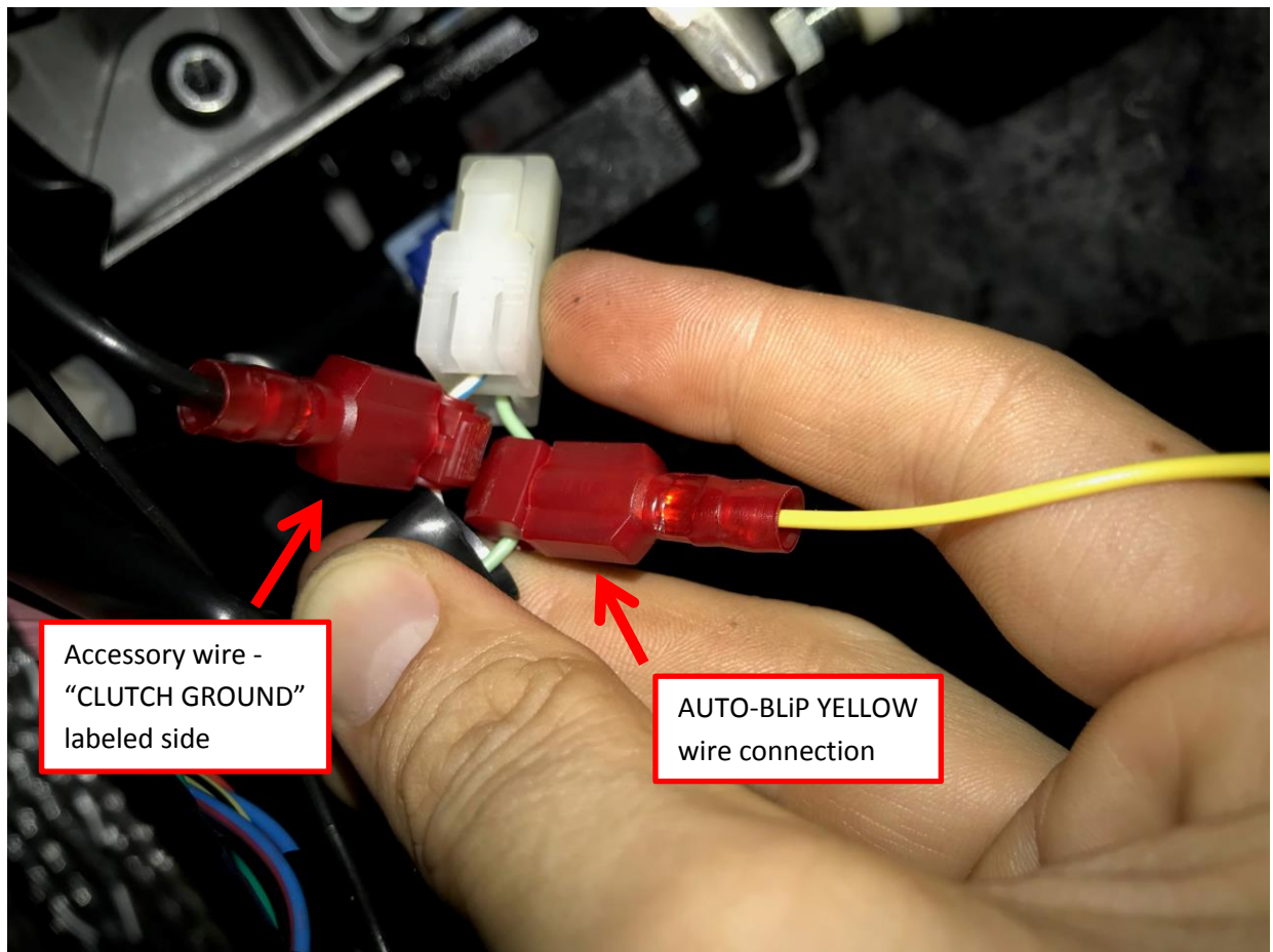
Figure 8 (Clutch pedal sensor T-tap connections)
