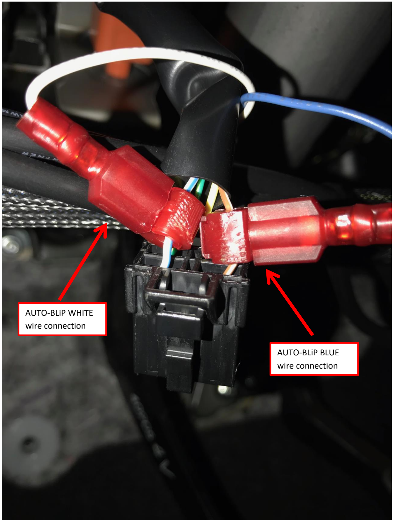
Figure 7 (Brake pedal sensor T-tap connections)
