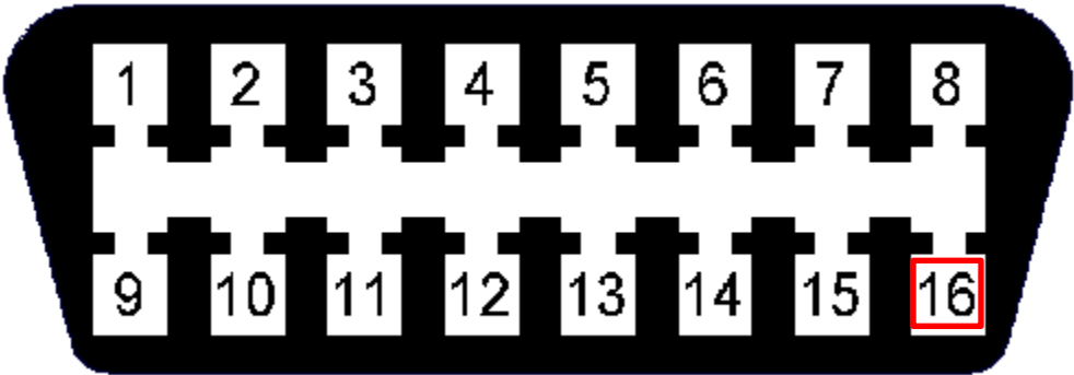
Figure 8 (OBD 2 Connector)
