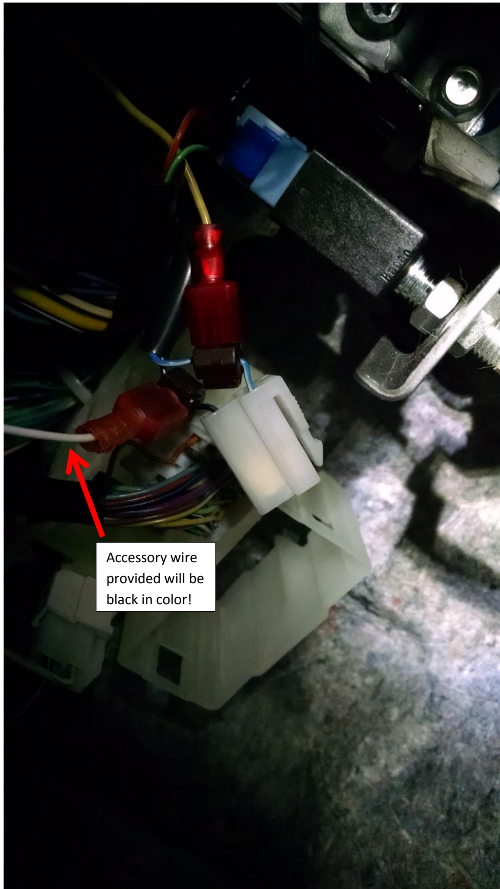
Figure 8 (Clutch pedal sensor T-tap connections)
