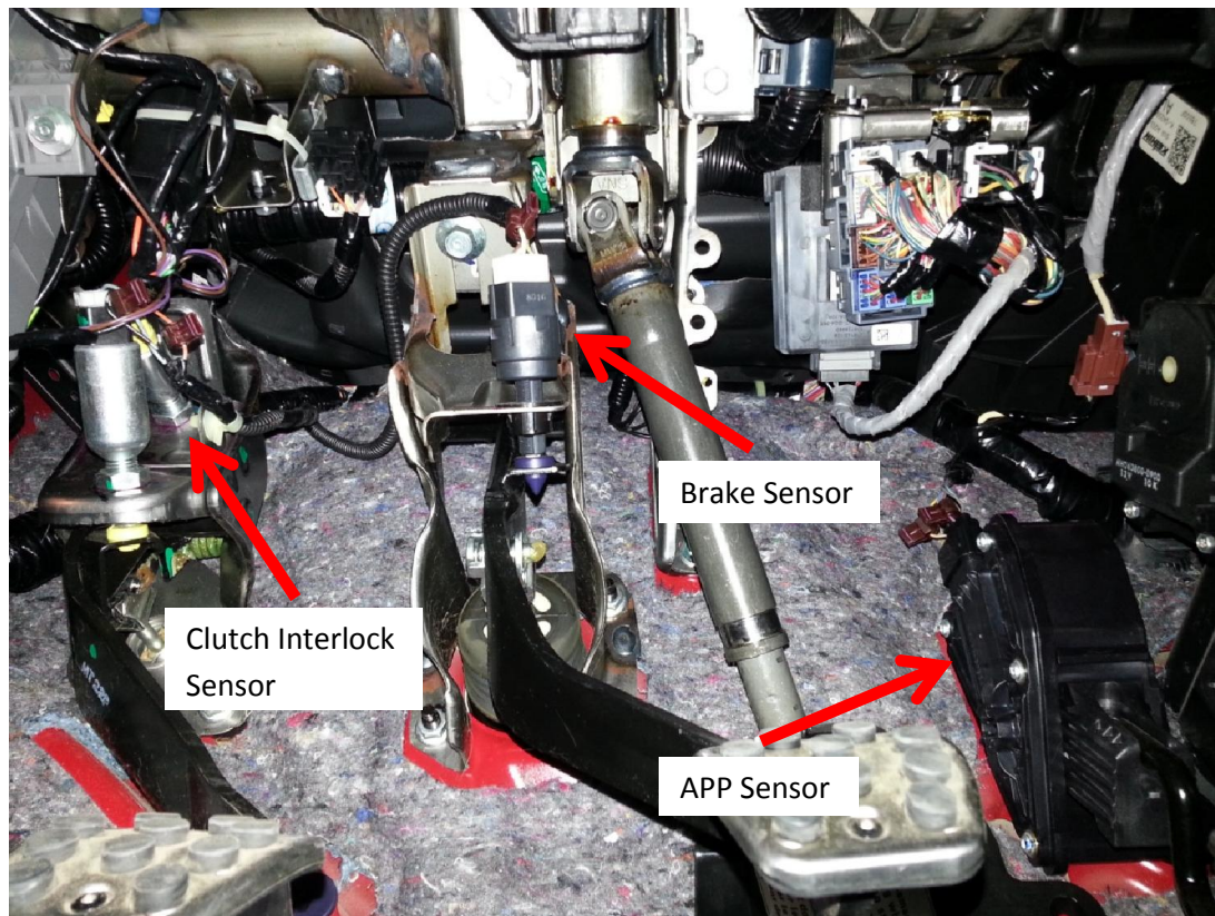
Figure 2 (Sensor locations)
