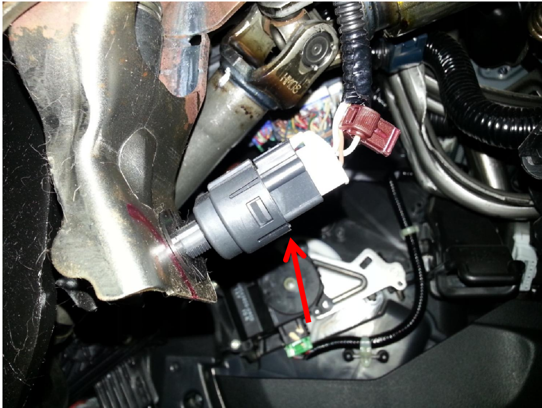
Figure 4 (Brake Sensor)
