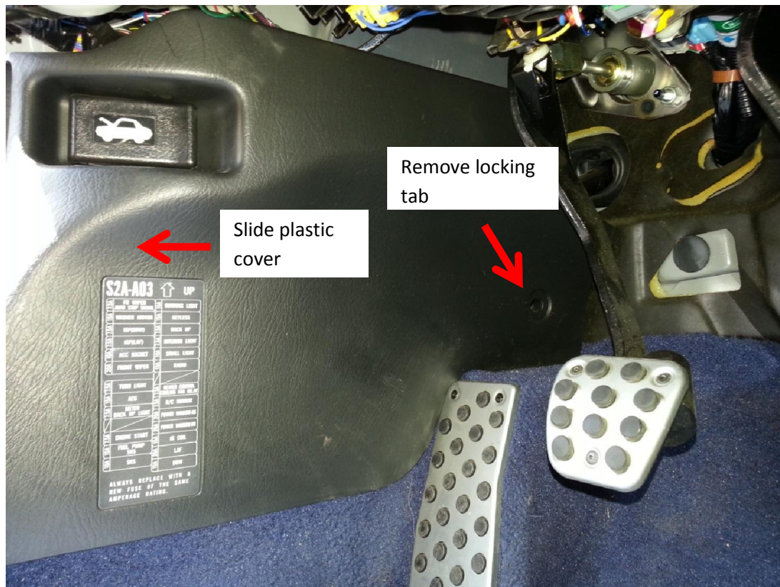
Figure 2 (ECU Location)
