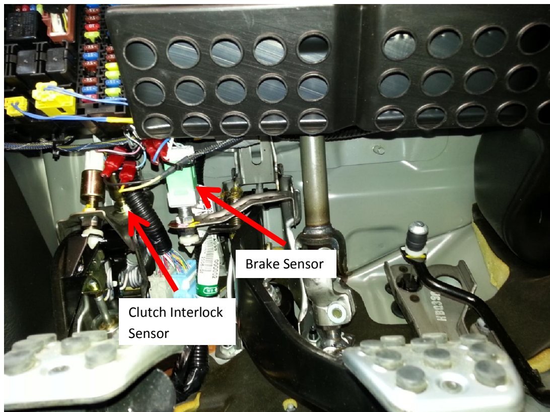
Figure 3 (Sensor Locations)
