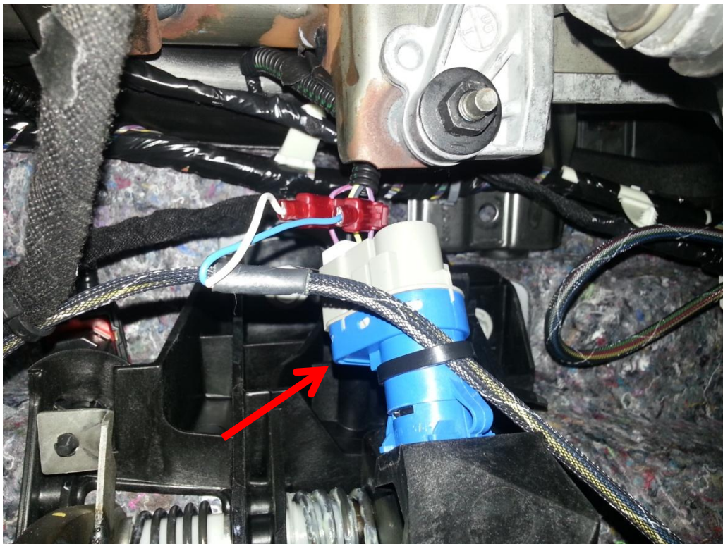
Figure 2 (Brake Sensor)
