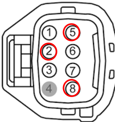
Accelerator Pedal Connector
