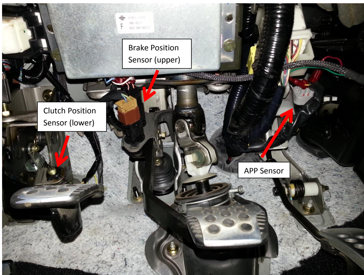
Figure 1 (Sensor Locations)
